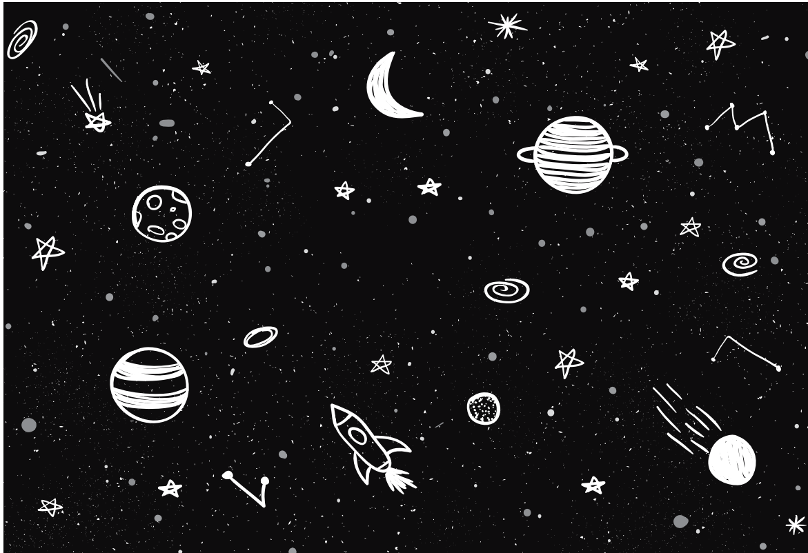
universe
